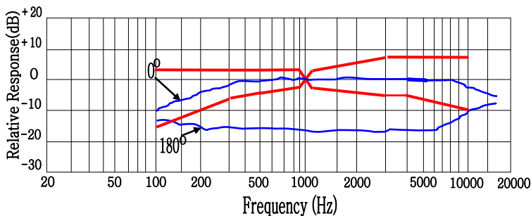
Frequency Response
