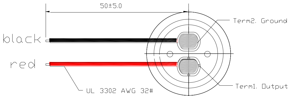
BOTTOM VIEW
