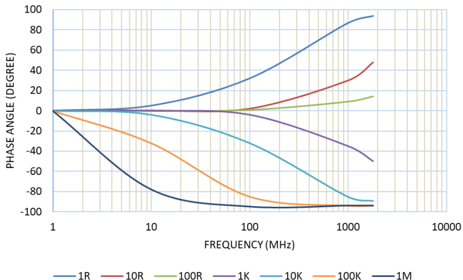
MLFA25 FREQUENCY x PHASE ANGLE
