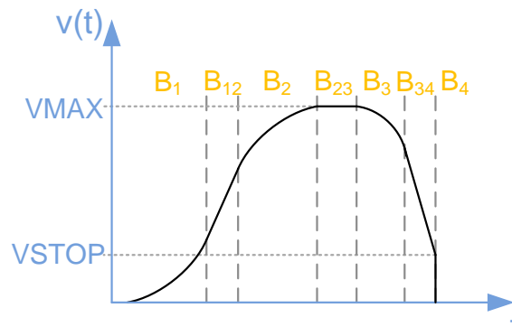
Figure 24: S-shaped Ramp with Stop Velocity
