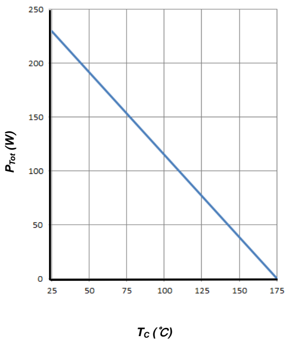
Figure 3. Power Derating
